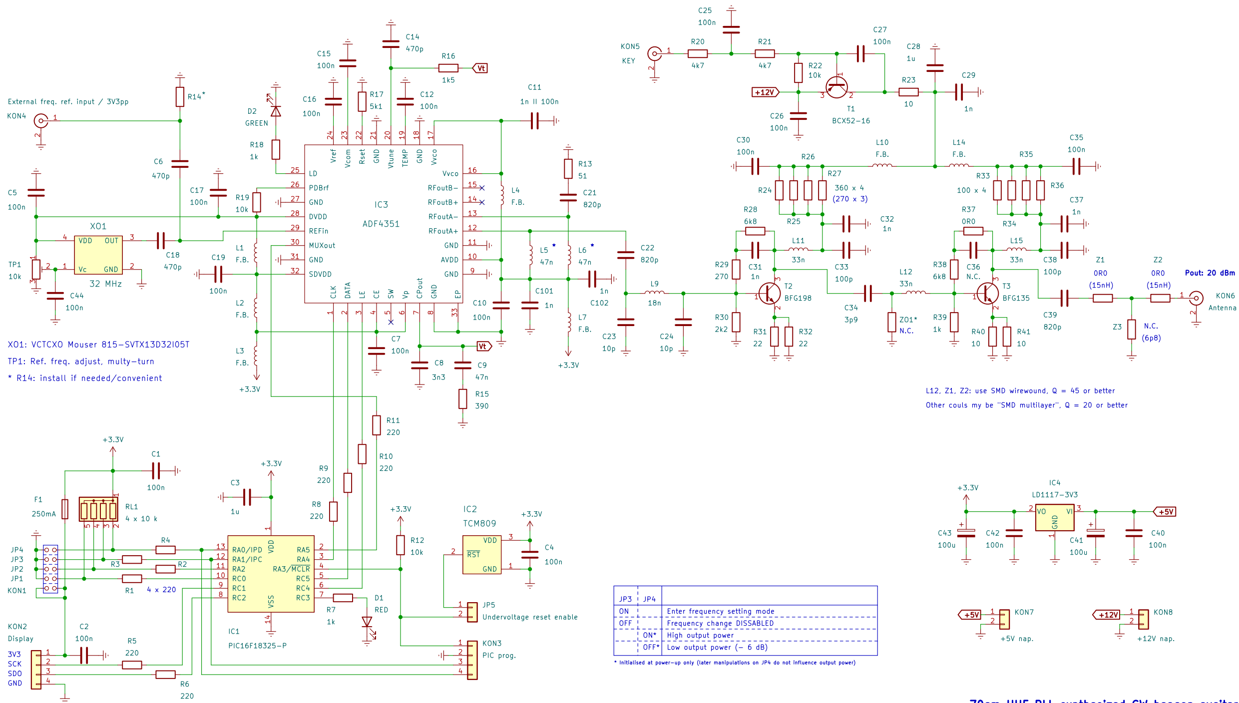
70cm UHF PLL synthesized CW beacon exciter S56AL, december 2019
